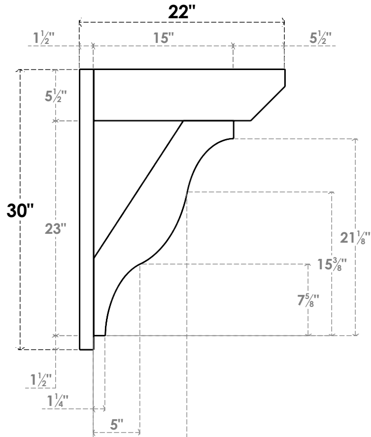
SIDE PROFILE
